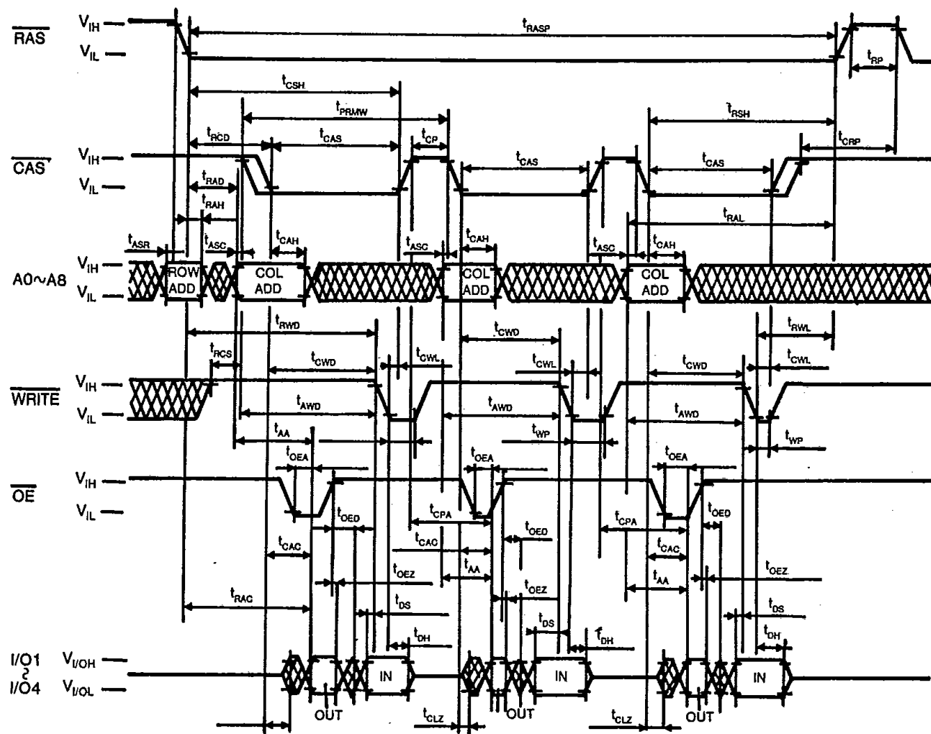
Figure 8. Fast Page Mode Read-Modify-Write Cycle
